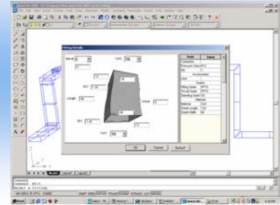
Edit Fitting
